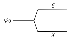
FIG. 2: The standard picturing of the double-slit experiment
